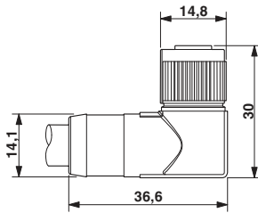
Dimensioned drawing
