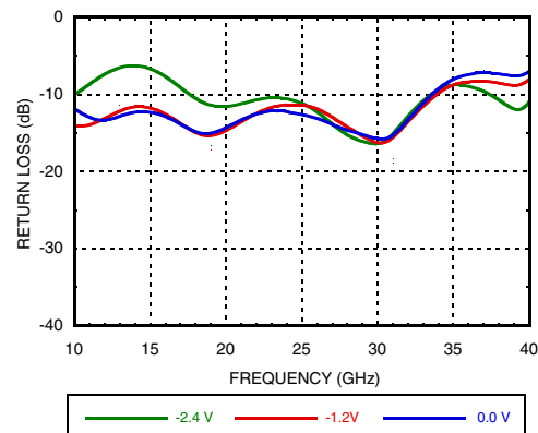
Output Return Loss Vctl1 = 0V, Vctl2 = Variable
