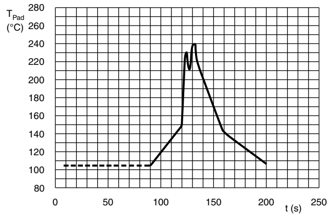
Fig. 6 - Maximum temperature load during (double-) wave soldering
