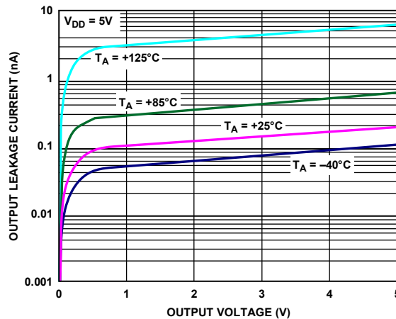
Figure 27. Output Leakage Current
