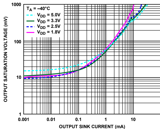
Figure 25. Output Saturation Voltage vs. Output Sink Current
