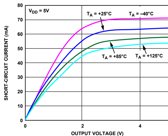
Figure 26. Output Short-Circuit Current
