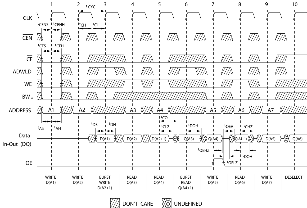
Figure 7. Read/Write/Timing [22, 23, 24]
