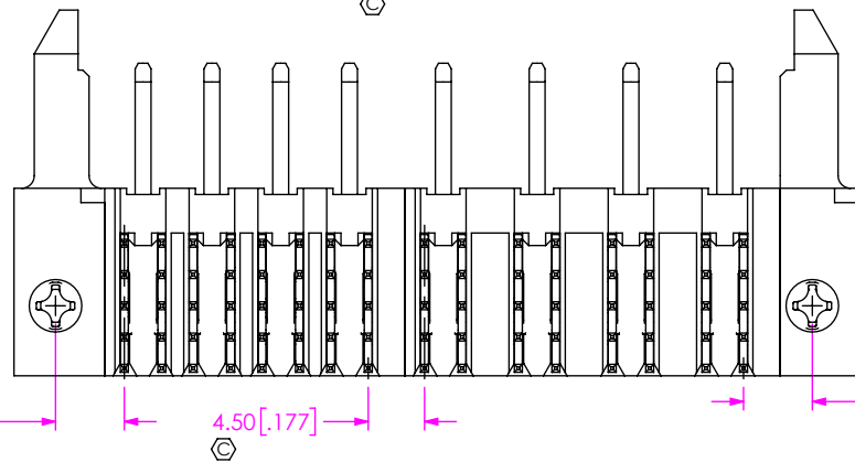
FIG 7 ET60T-D04-0-00-A04-X-R1-S SHOWN (DIFFERENT AS SHOWN, OTHERWISE SAME AS FIG 1)
