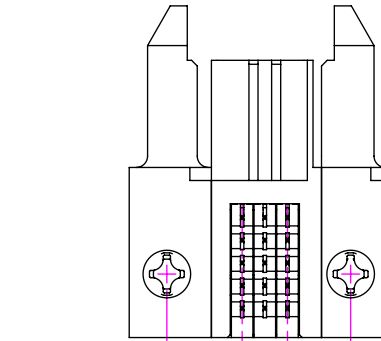
FIG 15 ET60T-000-5-03-000-X-RX-S SHOWN (DIFFERENT AS SHOWN, OTHERWISE SAME AS FIG 4)
