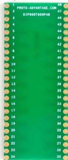
2D Top View (Pins Unassembled)
