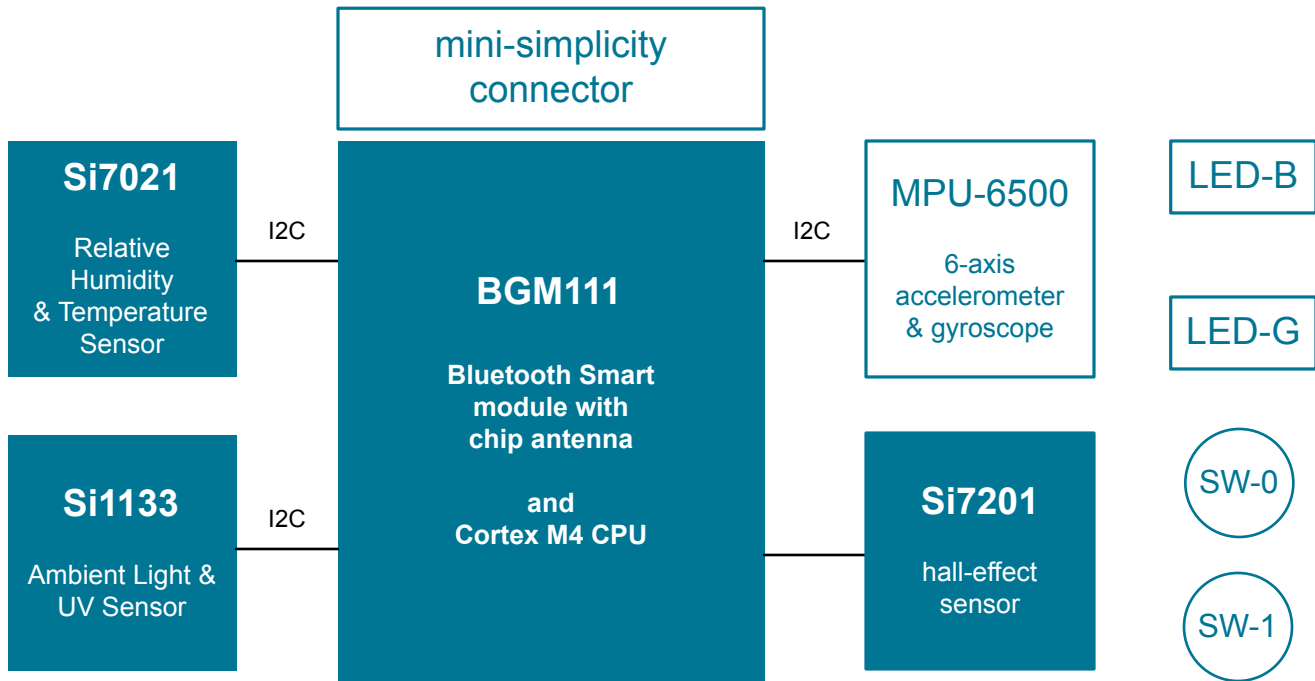
Figure 5.1. Hardware Block Diagram
