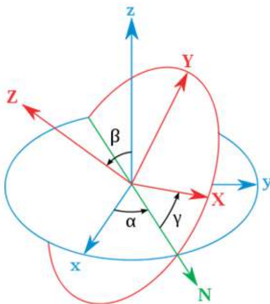
Figure 6.2. Orientation Representation
