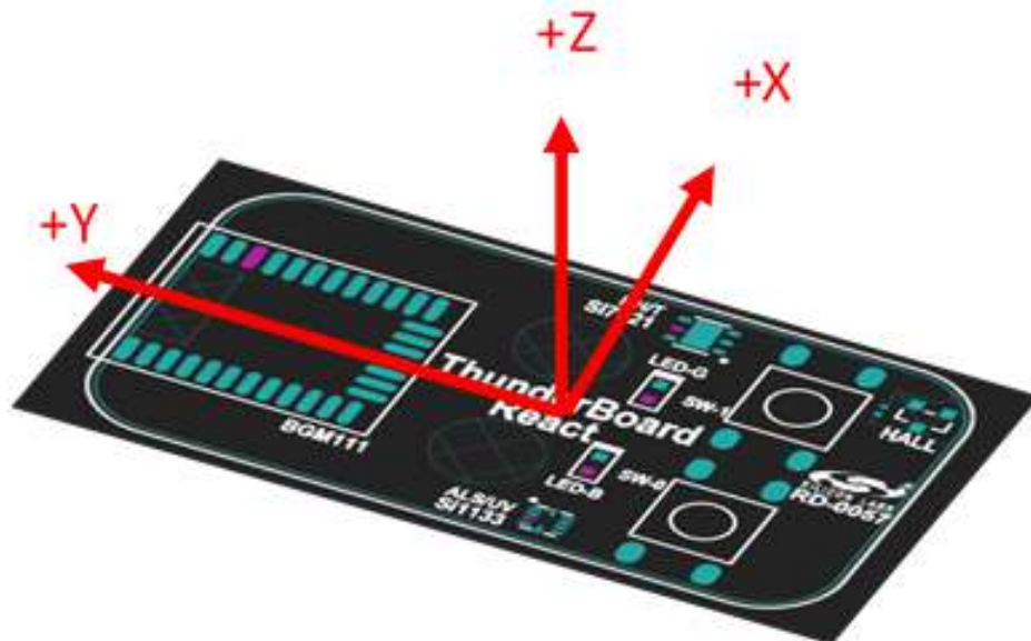
Figure 6.1. Hardware Axis Orientation
