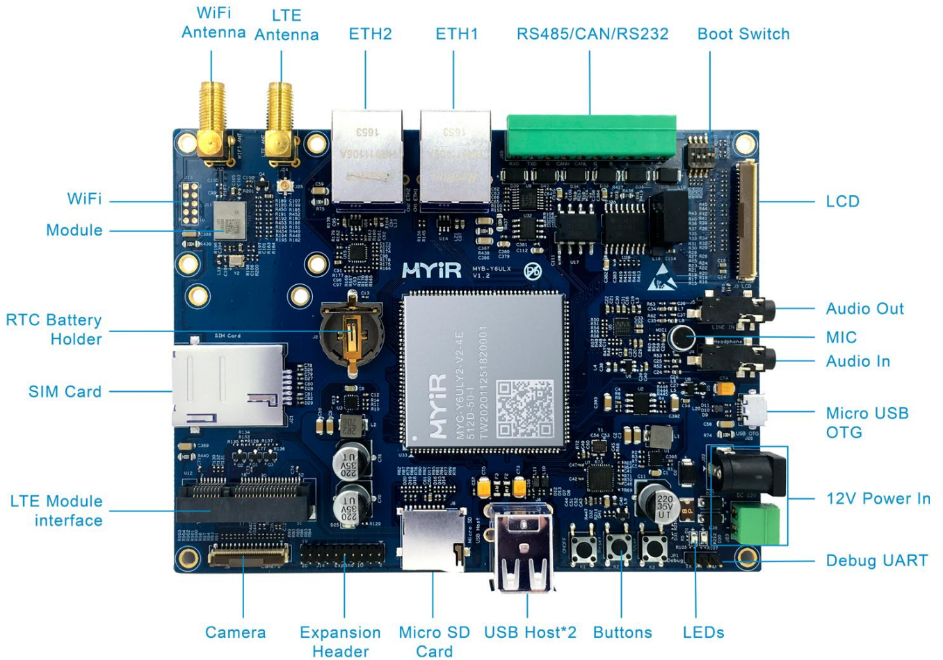
MYD-Y6ULX-V2 Development Board
