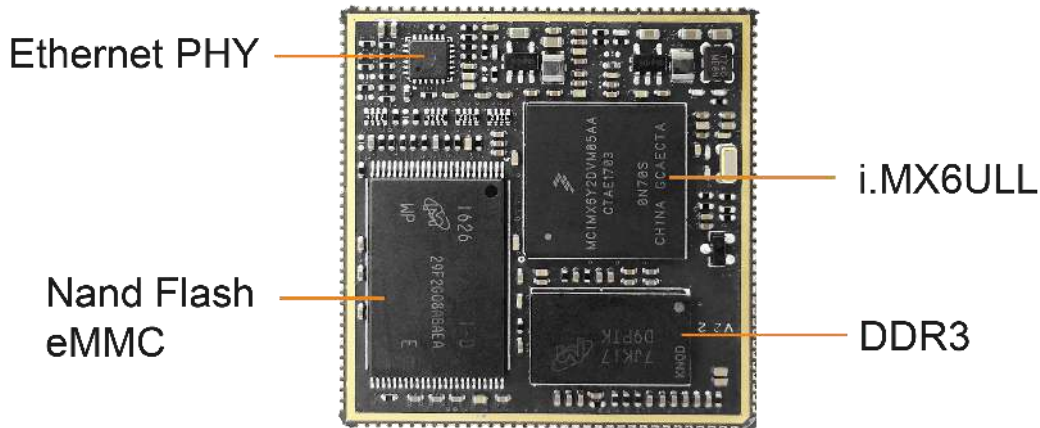
MYC-Y6ULX-V2 CPU Module Top-view (delivered with shielding cover by default)
