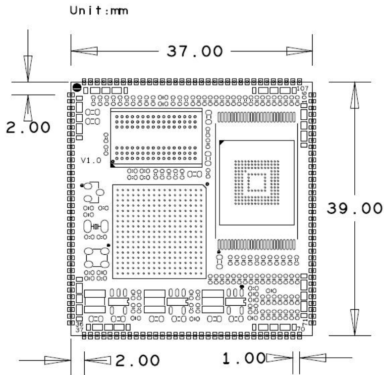
MYC-Y6ULX-V2 Dimension Chart
