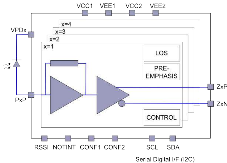
Figure 1: Device diagram
