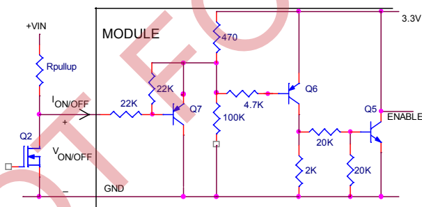
Circuit configuration for using positive On/Off logic.
