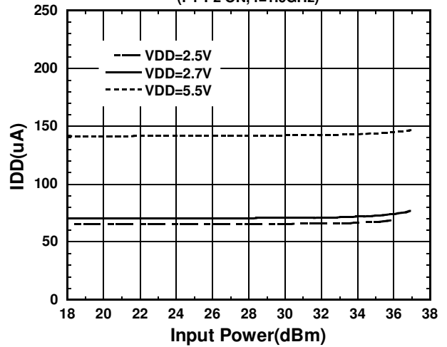
IDD vs. Input Power (P1-P2 ON, f=1.9GHz)
