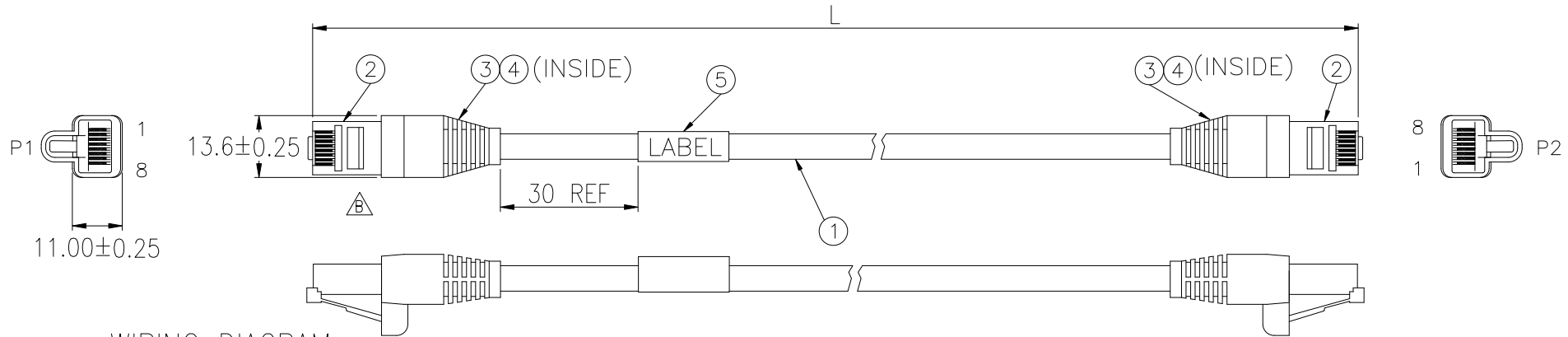
WIRING DIAGRAM
