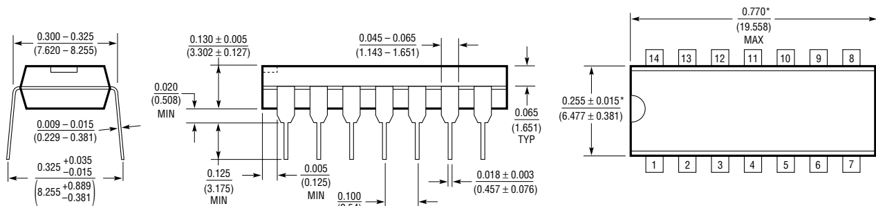
N Package 14-Lead PDIP (Narrow 0.300) (LTC DWG # 05-08-1510)
