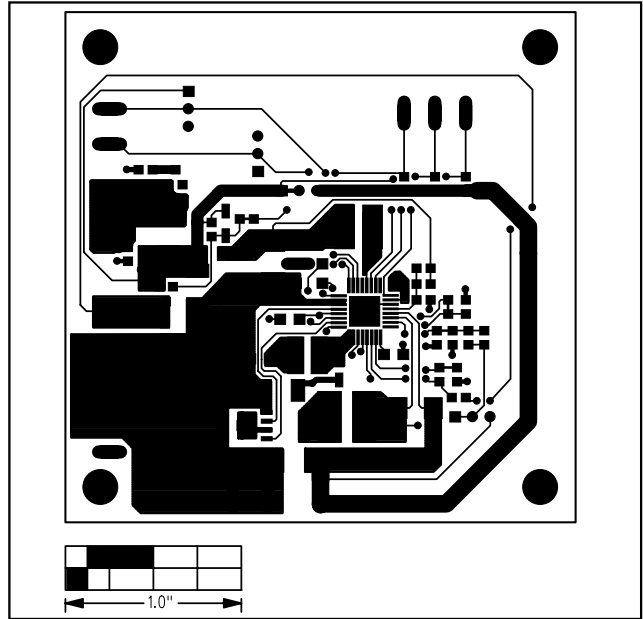
Figure 3. MAX1774 EV Kit PC Board Layout—Component Side
