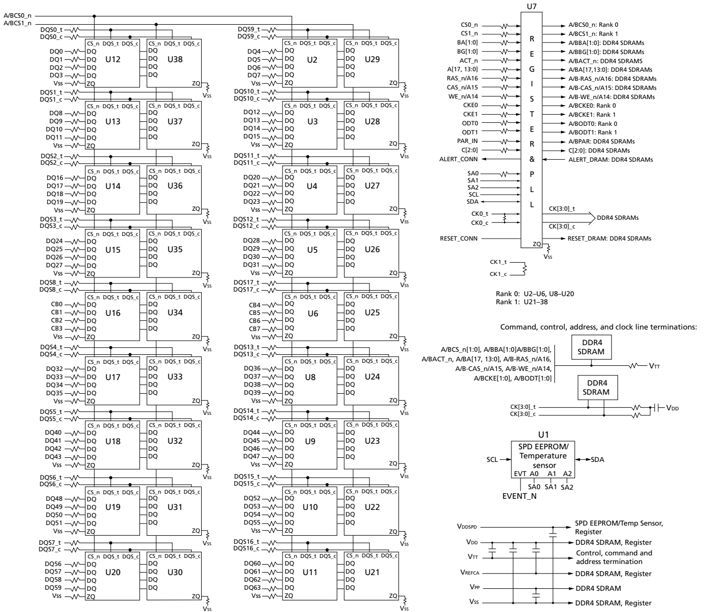
Figure 4: Functional Block Diagram, R/C-B2 (PCBs 1971, 2436, or 2615)
