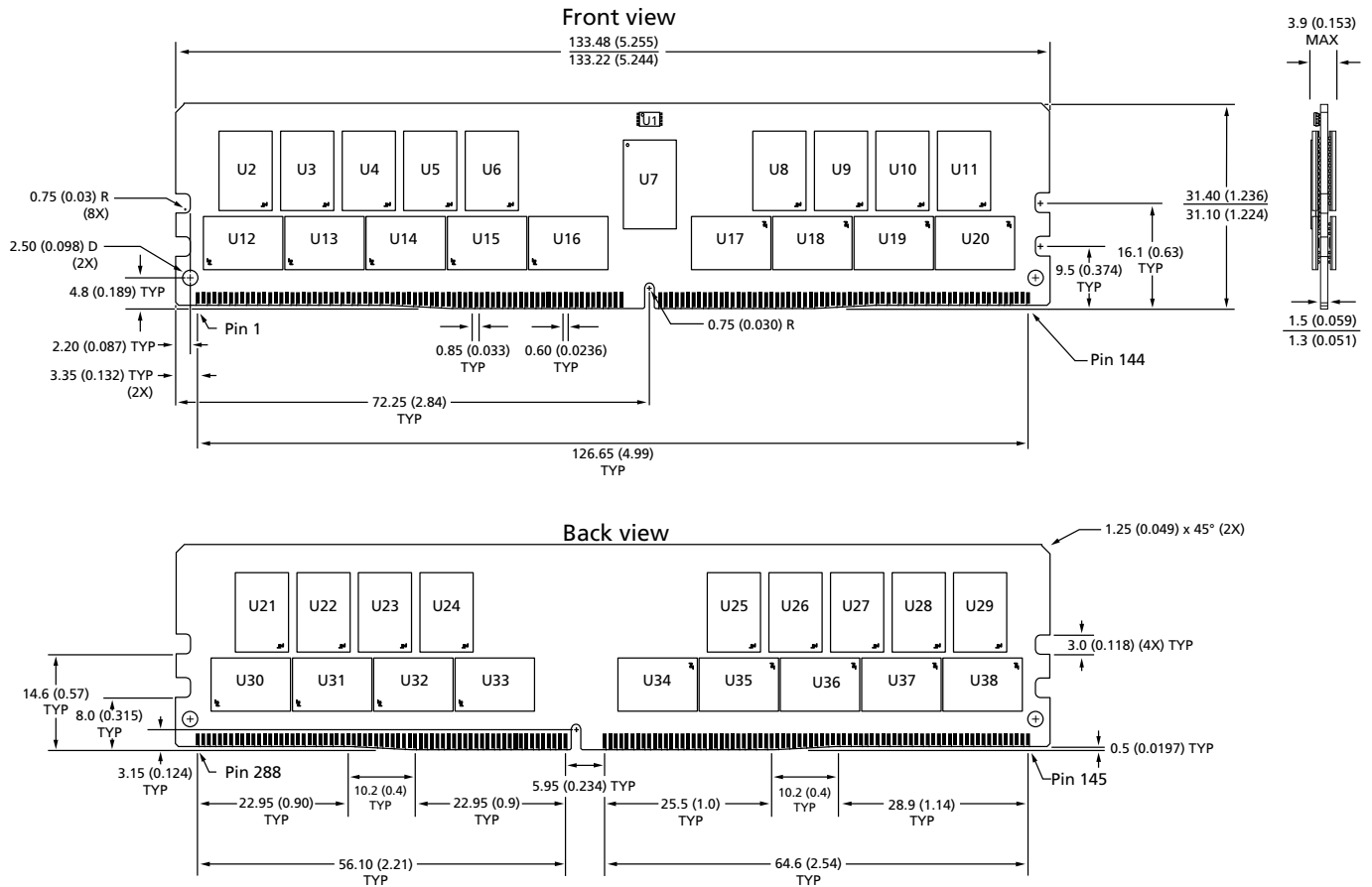
Figure 6: 288-Pin DDR4 RDIMM (R/C-B2, PCBs 1971, 2436, or 2615)
