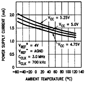
Power Supply Current (I CC ) vs Ambient Temperature
