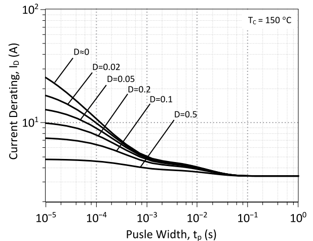
Figure 18: Drain Current Derating vs. Pulse Width
