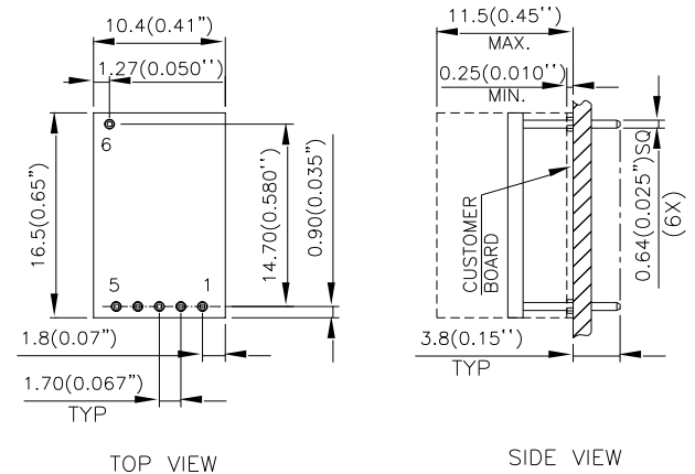
PIN ASSIGNMENT
