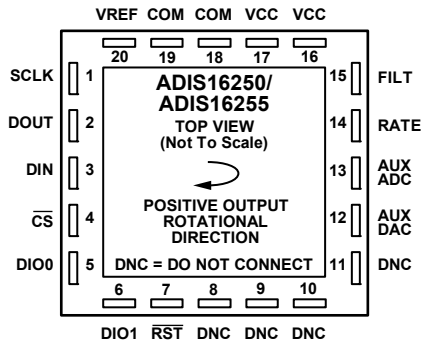
Figure 5. Pin Configuration
