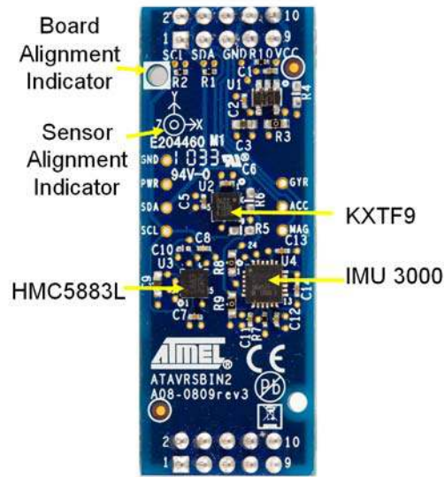
Figure 4-1. Sensor arrangement.
