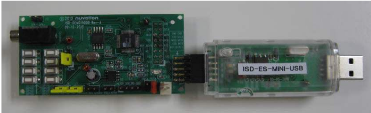
Figure 3 – ISD_DEMO15D00 connected with ISD-ES_MINI_USB (dongle) board
