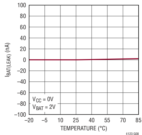
Battery Leakage Current vs Temperature
