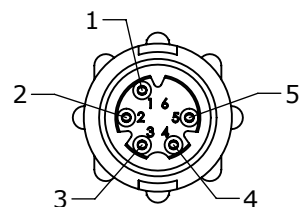
FACE VIEW 18980-5SG-5XX 5 POSITION A-KEY
