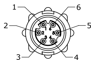
FACE VIEW 18980-6SG-5XX 6 POSITION B-KEY
