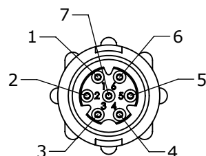
FACE VIEW 18980-7SG-5XX 7 POSITION A-KEY
