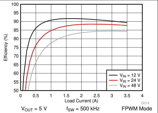
Figure 26. LM76003 Efficiency
