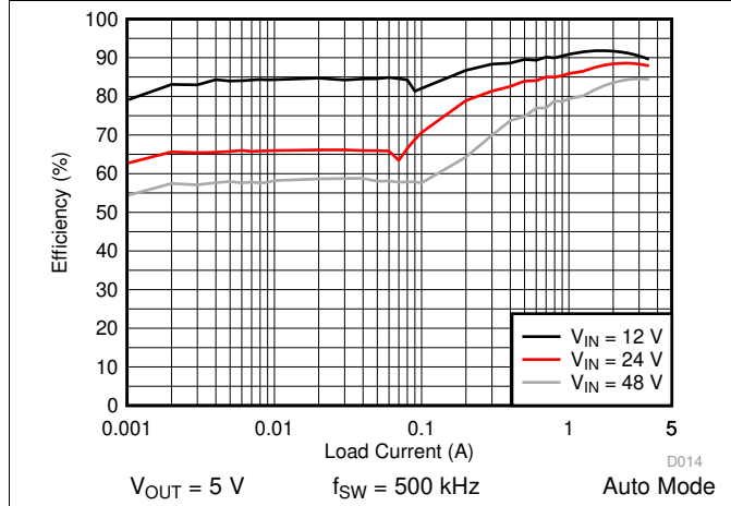
Figure 25. LM76003 Efficiency
