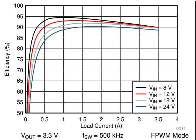
Figure 24. LM76003 Efficiency
