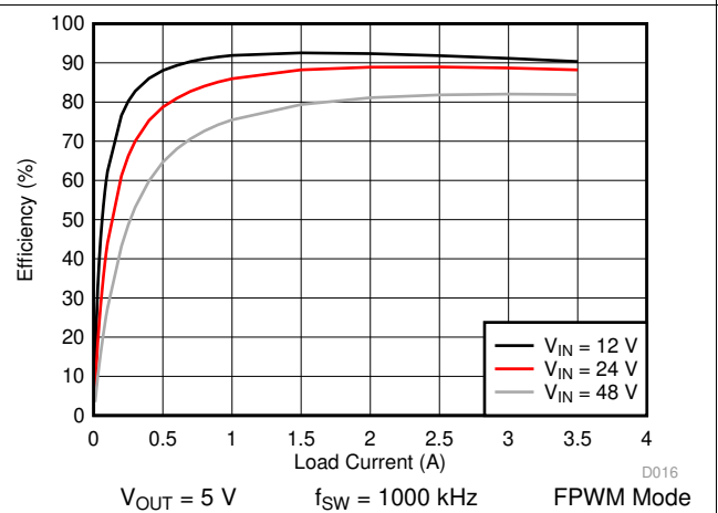
Figure 28. LM76003 Efficiency
