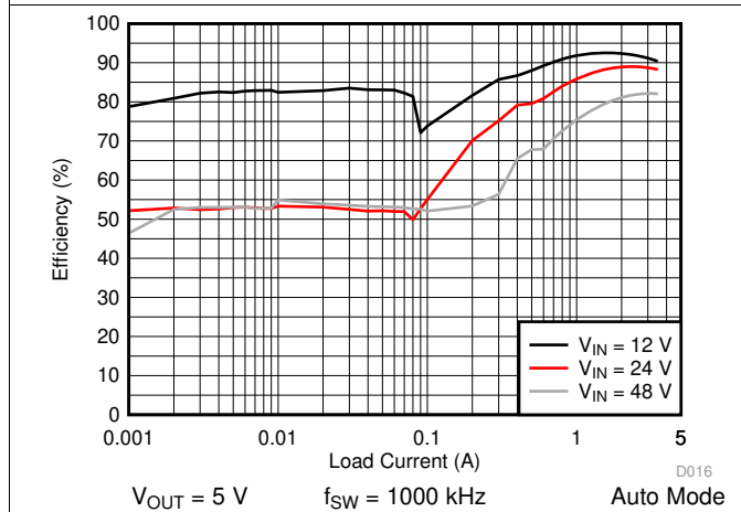
Figure 27. LM76003 Efficiency
