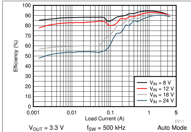
Figure 23. LM76003 Efficiency
