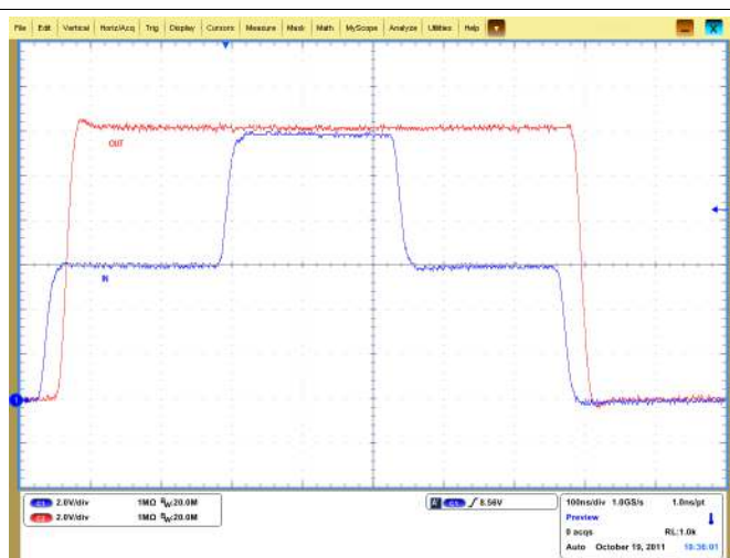
Figure 36. Step Input
