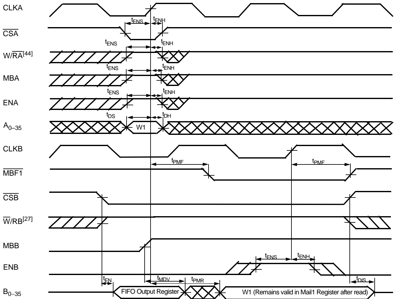
Timing for Mail1 Register and MBF1 Flag (CY Standard and FWFT Modes) [43,45]
