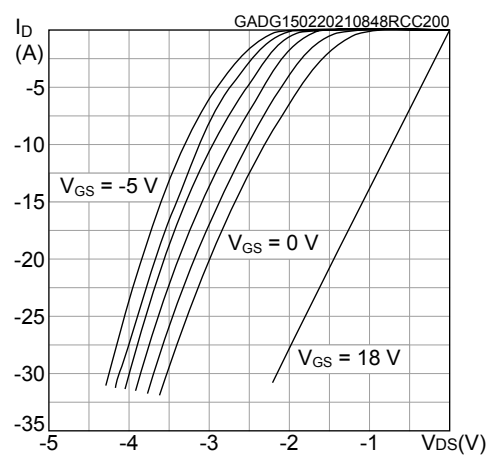
Figure 16. Typical reverse conduction characteristics ( T_J = 200\text{ °C} )
