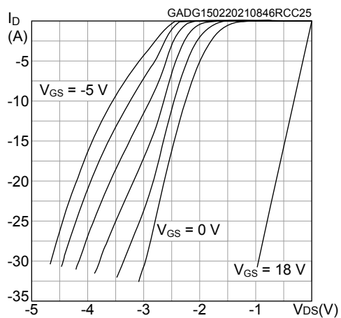
Figure 15. Typical reverse conduction characteristics ( T_J = 25\text{ °C} )
