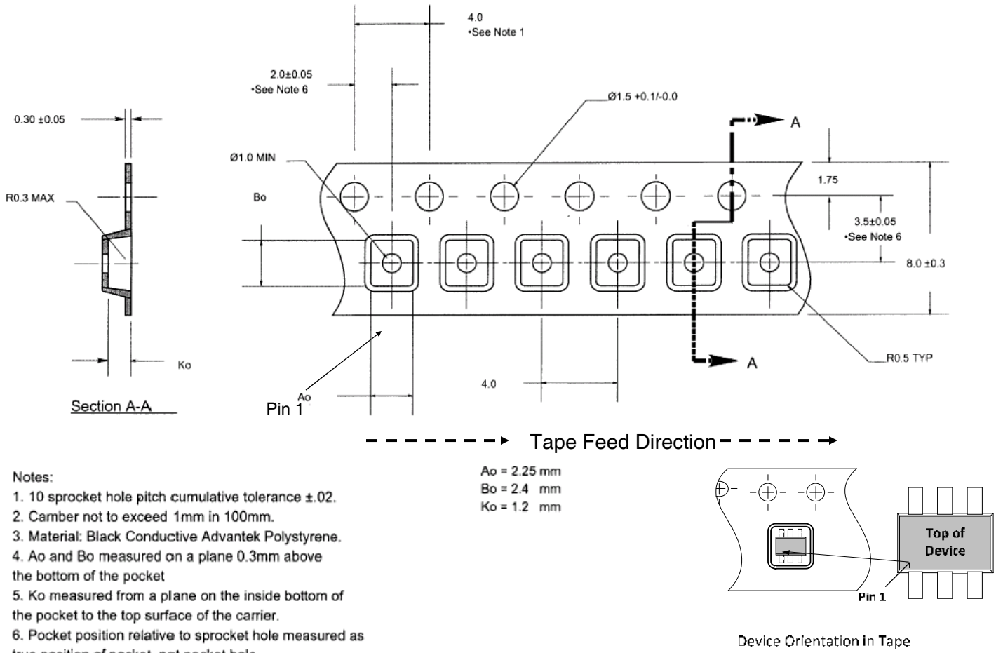
Figure 16. Tape and Reel Specifications
