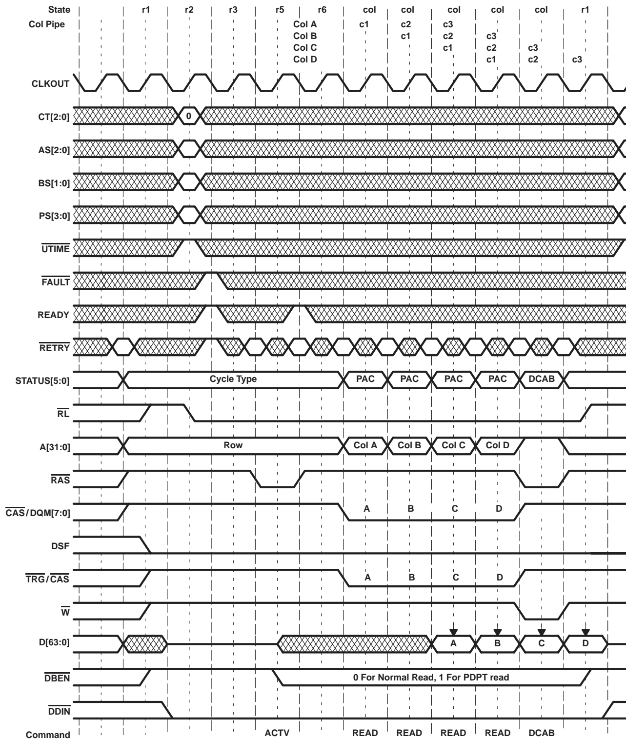
Figure 94. SDRAM Burst-Length 1, 2 Cycle Latency Read-Cycle Timing
