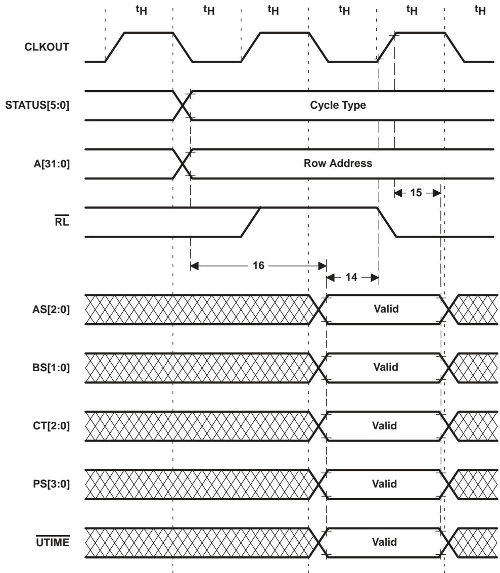
Figure 121. Local Bus Timing: Cycle Configuration Inputs
