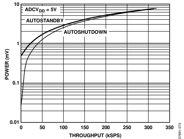
Figure 73. Power vs. Throughput Rate in Autoshutdown and Autostandby Mode
