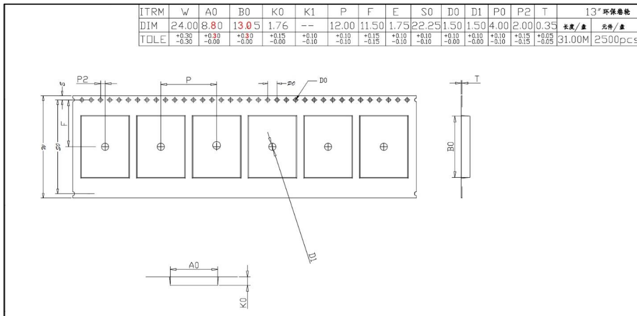
Figure 21: Tape specifications
