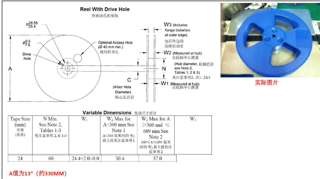
Figure 20: Reel specifications
