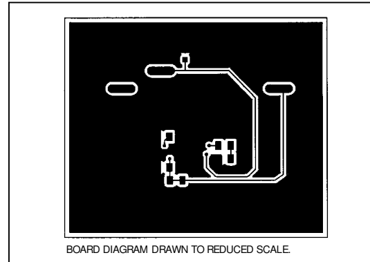
Figure 5. PC Board Layout—Solder Side
