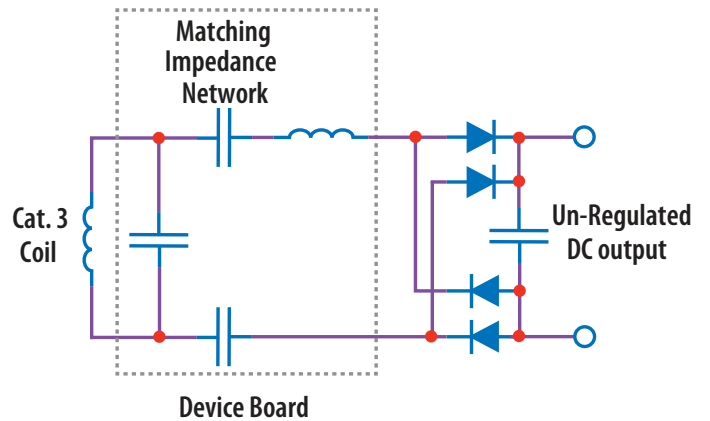
Figure 5: Basic schematic of the AirFuel Category 3 device board.
