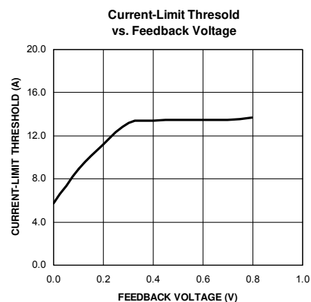
Figure 4. MIC26400 Current Limit Foldback Characteristic
