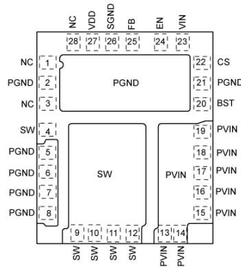
28-Pin 5mm X 6mm MLF® (YJL)
