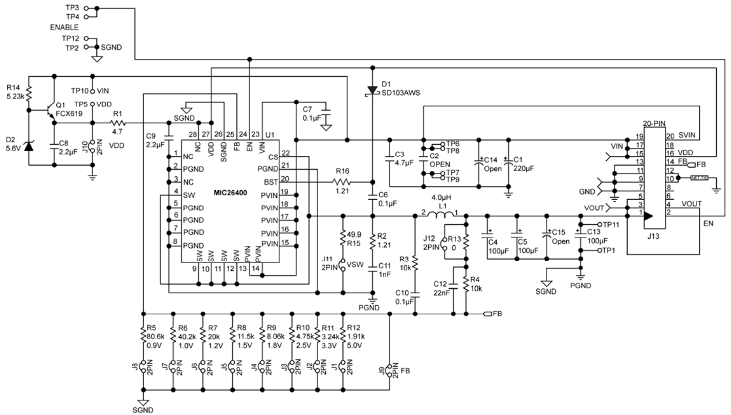
Figure 8. Schematic of MIC26400 Evaluation Board (J13, R13, R15 are for testing purposes)
