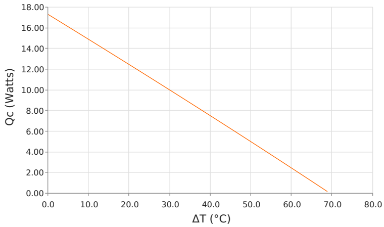
Heat Pumped at Cold Side (Qc) Thot = 27 °C | Current = 3.4 Amps
