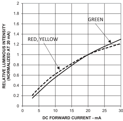
Figure 3: Relative luminous intensity vs. DC forward current (HLMP-4015, HLMP-08xx)
