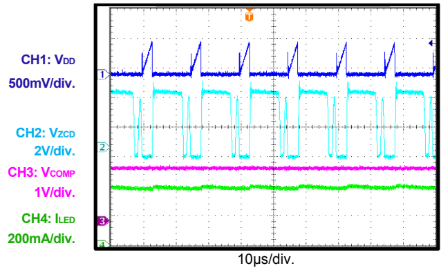
Steady State V_{IN}=230Vac , 7 LED Output
