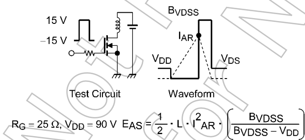
Fig. 8.16 Test Circuit/Waveform
