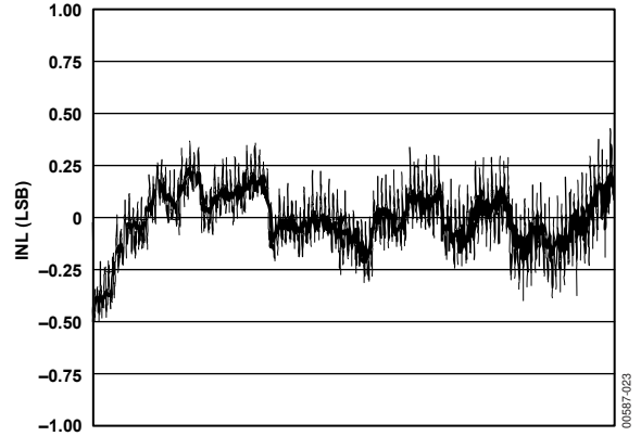
Figure 19. Integral Nonlinearity, f_s = 105 MSPS
