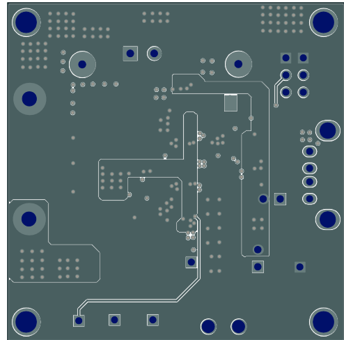
Figure 4: Mid Layer2
