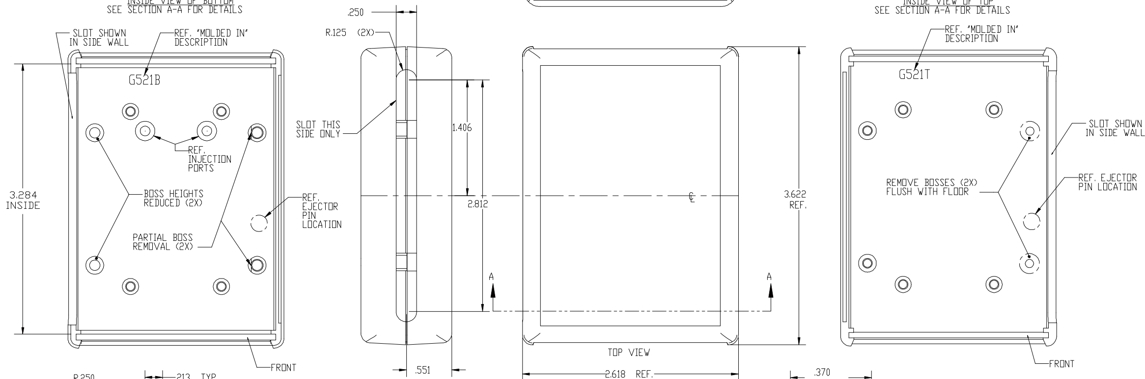
VIEW 1 INSIDE VIEW OF BOTTOM SEE SECTION A-A FOR DETAILS
