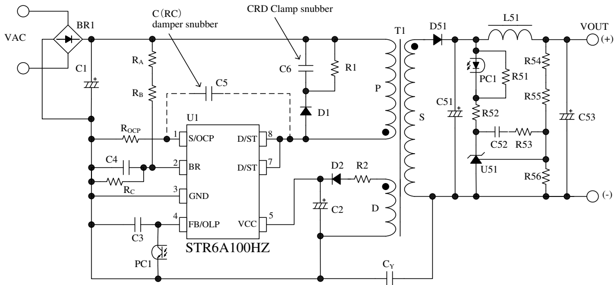
Figure6-1 Typical application circuit (enabled Brown-In/Brown-Out Function, DC line detection)
