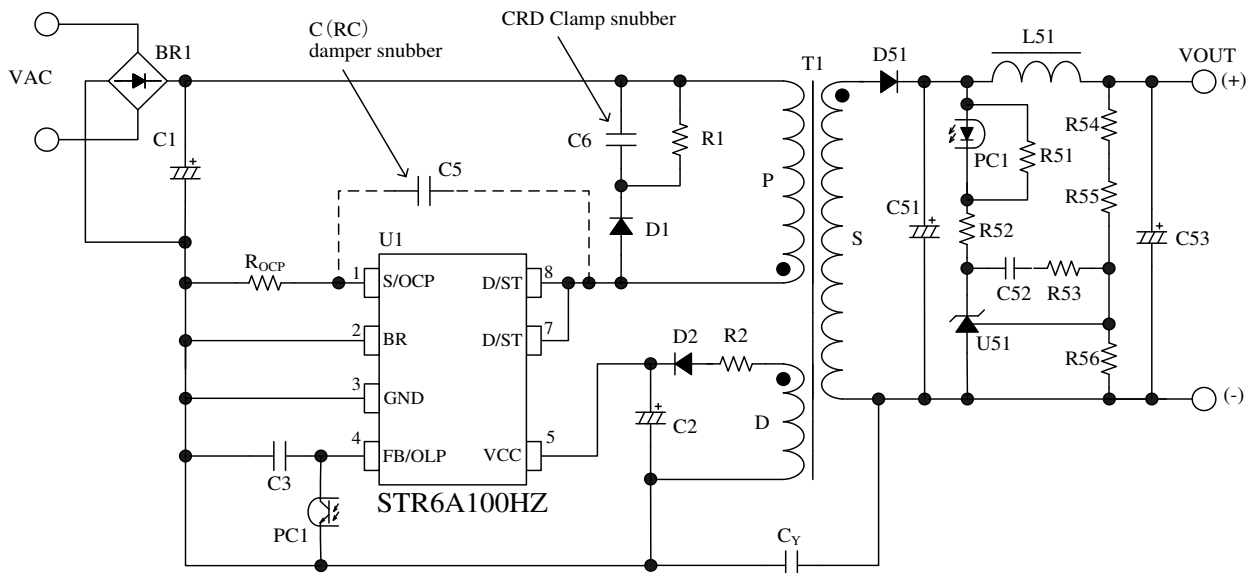
Figure6-1 Typical application circuit (enabled Brown-In/Brown-Out Function, DC line detection)
