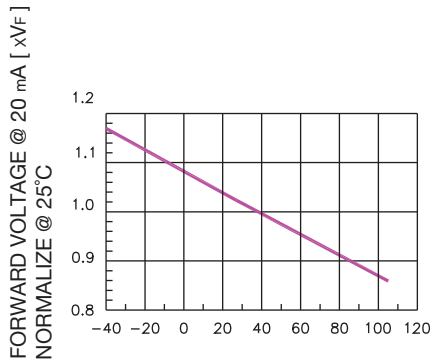
AMBIENT TEMPERATURE T_a (°C) FORWARD VOLTAGE VS. TEMPERATURE
