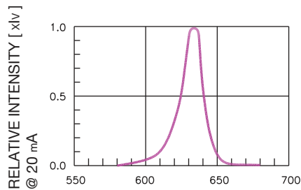
WAVELENGTH (nm) RELATIVE INTENSITY VS. WAVELENGTH
