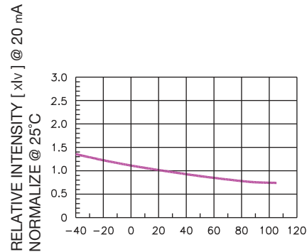
AMBIENT TEMPERATURE T_a (°C) RELATIVE INTENSITY VS. TEMPERATURE
