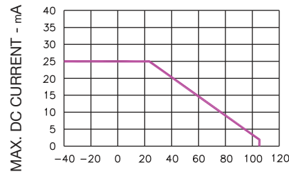
AMBIENT TEMPERATURE T_a (°C) MAX. ALLOWABLE DC CURRENT VS. AMBIENT TEMPERATURE
