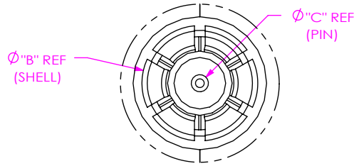
DETAIL 'A' SCALE 8:1
