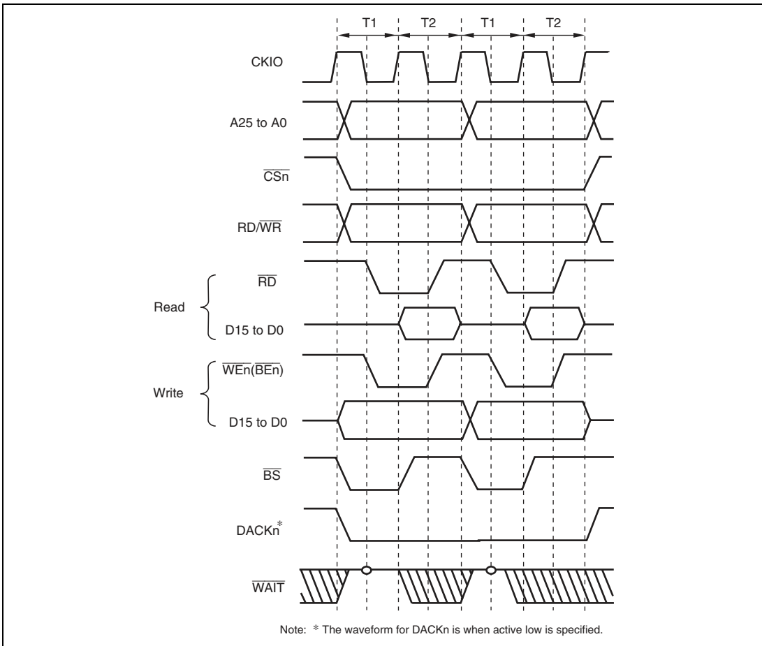
Figure 12.5 Continuous Access for Normal Space 2, Bus Width = 16 bits, Longword Access, \overline{CS}_n\overline{WCR.WM} Bit = 1 (Access Wait = 0, Cycle Wait = 0)
