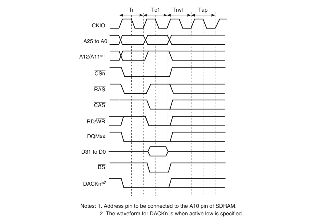
Figure 12.18 Basic Timing for Single Write (Auto-Precharge)
