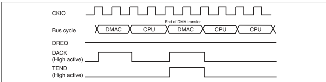
Figure 13.16 Example of DMA Transfer End Timing (Cycle Steal Level Detection)
