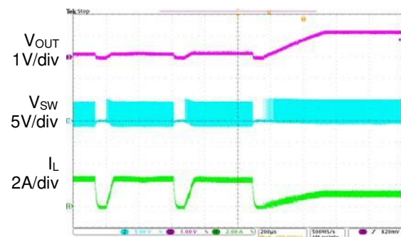
Time 200µs/div
