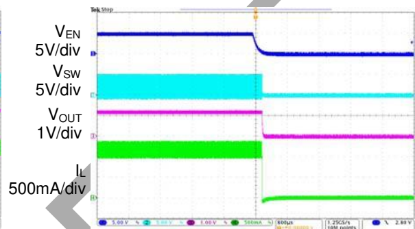
Time 800µs/div
