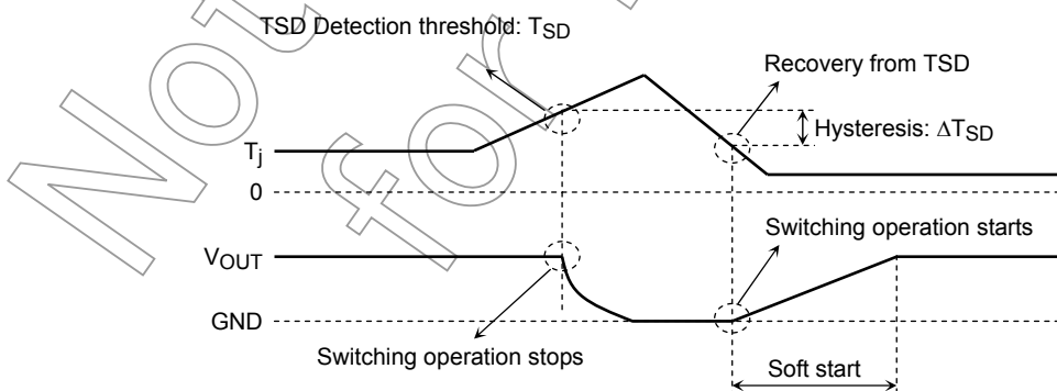
Figure 5 Thermal Shutdown Operation
