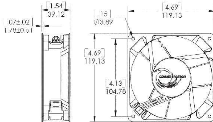
MECHANICAL DRAWING
