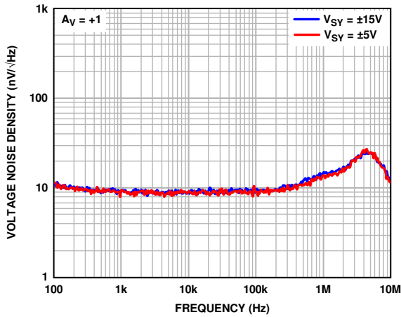
Figure 64. Voltage Noise Density vs. Frequency, V_{SV} = \pm 5V and V_{SV} = \pm 15V
