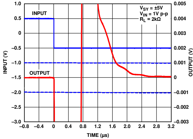
Figure 63. Negative Settling Time to 0.1%, V_{SV} = \pm 5V
