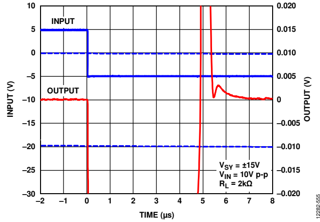
Figure 66. Negative Settling Time 0.1%, V_{SV} = \pm 15V
