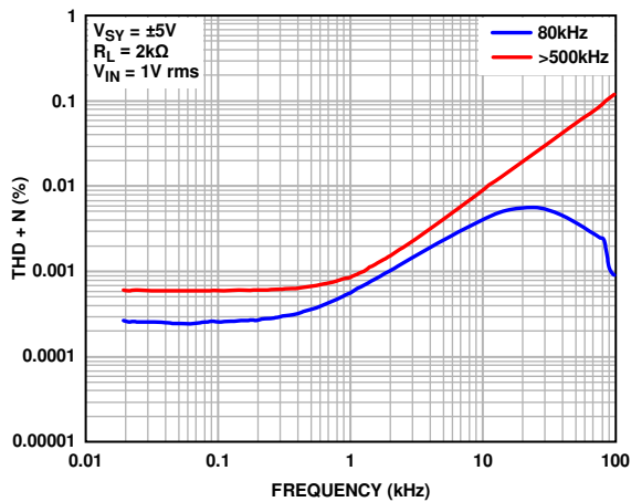
Figure 65. THD + N vs. Frequency, V_{SV} = \pm 5V
